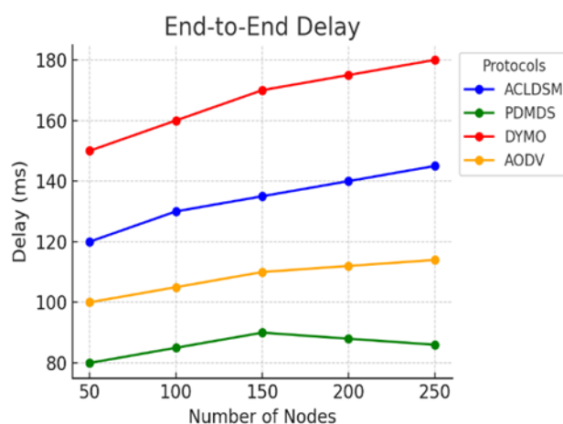
Figure 3 End to End Delay (EED): Comparison in Nodes Relating to Various Routing Protocols in Different Numbers
