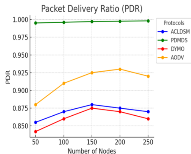
Figure 2 Packet Delivery Ratio (PDR): Comparison in Nodes Relating to Various Routing Protocols in Different Numbers
