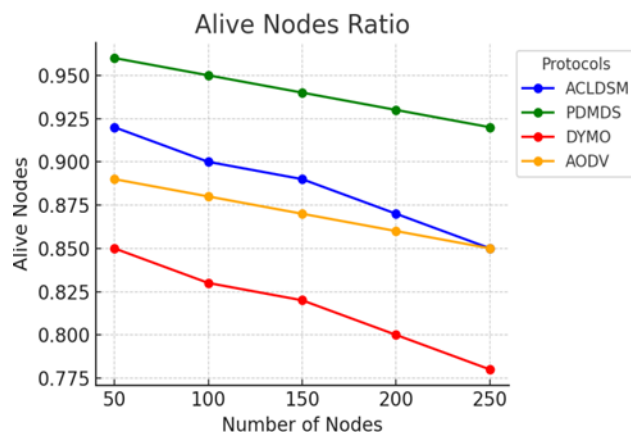
Figure 6 Alive Nodes Ratio: Comparison in Nodes Relating to Various Routing Protocols in Different Numbers
