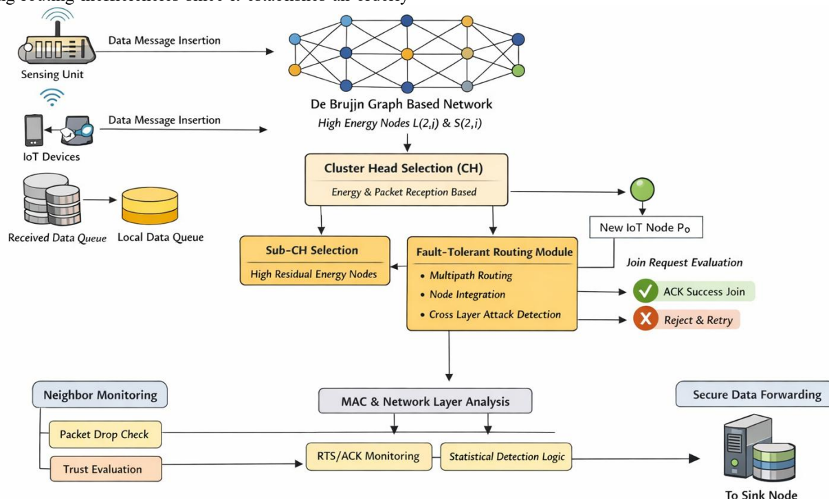
Figure 1 Proposed Framework Architecture for PDMDs-Based Secure Data Aggregation and Routing
